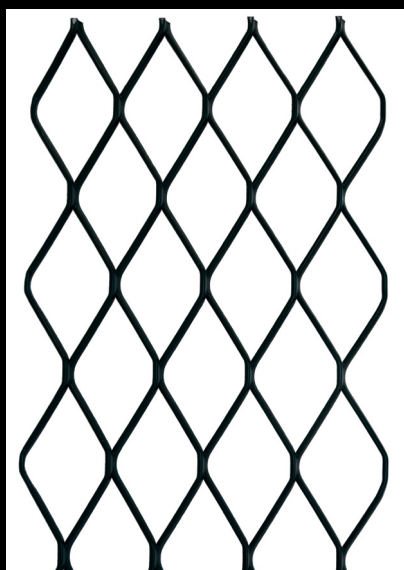
Mesh Ref: 4095 101.60 x 50.80 x 4.5 x 3.00 4.90KG/M2 white weight
