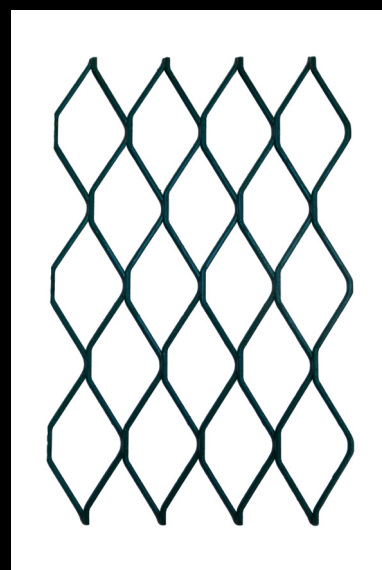
Mesh Ref: 3396 85.73 x 40.64 x 3.18 x 3.00 4.03KG/M2 white weight
